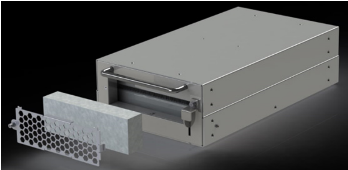
Figure 9. Front view of 7 kW rectifier, filter, retainer and dead metal
