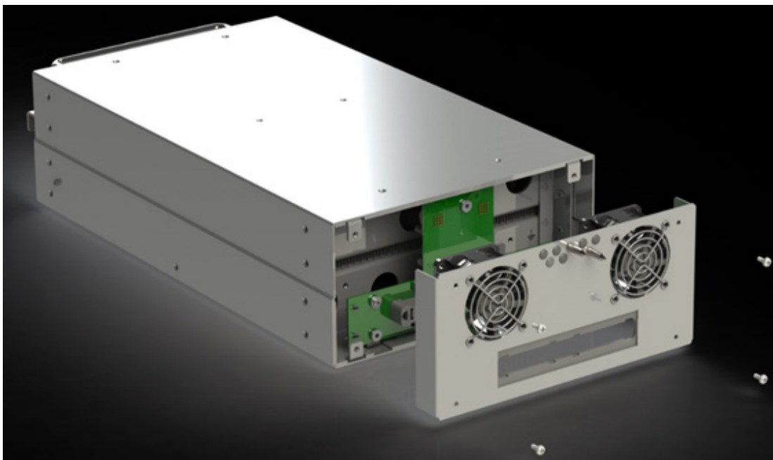
Figure 10. Rear view of 7 kW rectifier with fan subassembly
